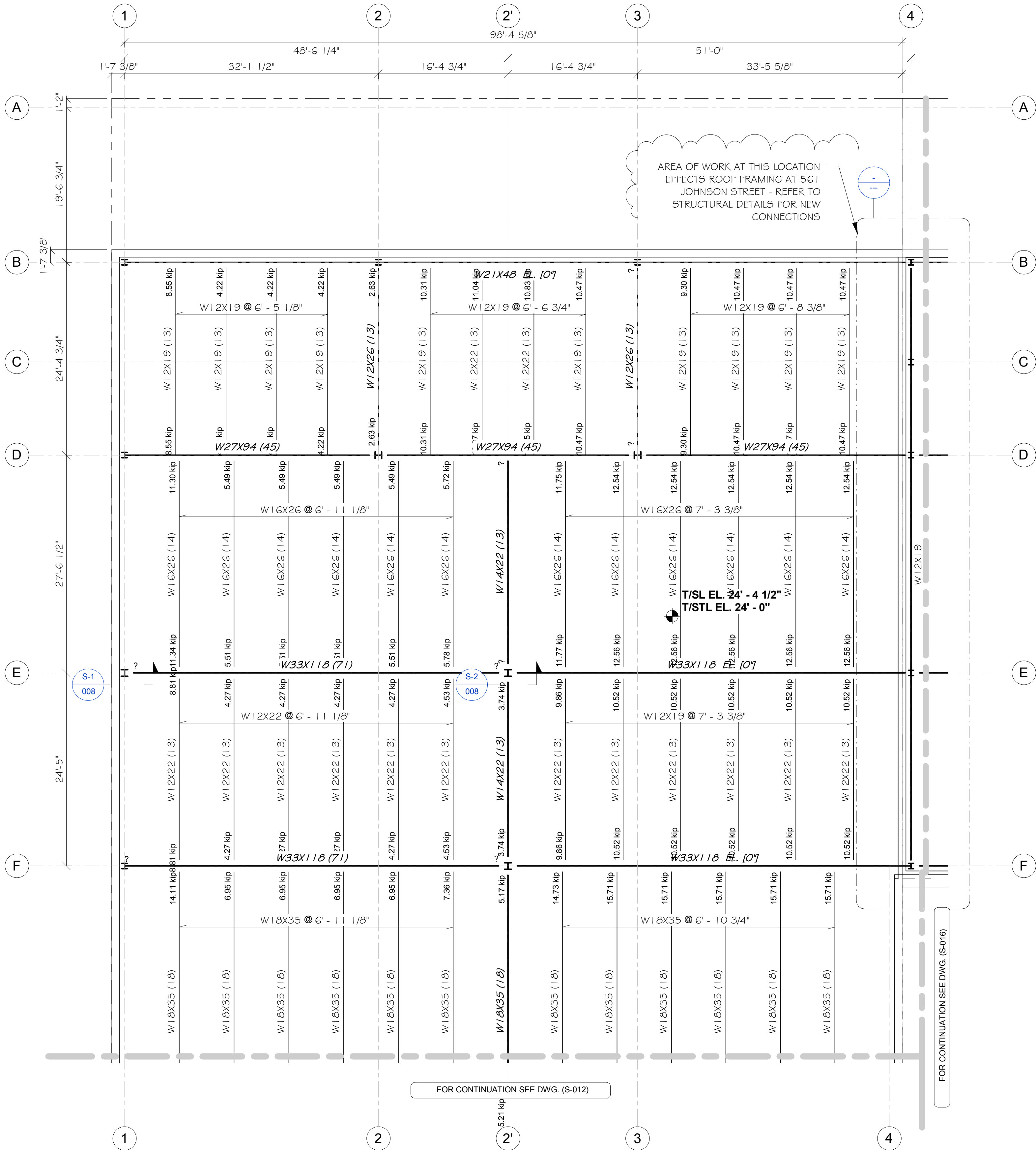
Partial - Proposed Roof Framing Plan @ 537 Johnson Ave (1 of 2):
