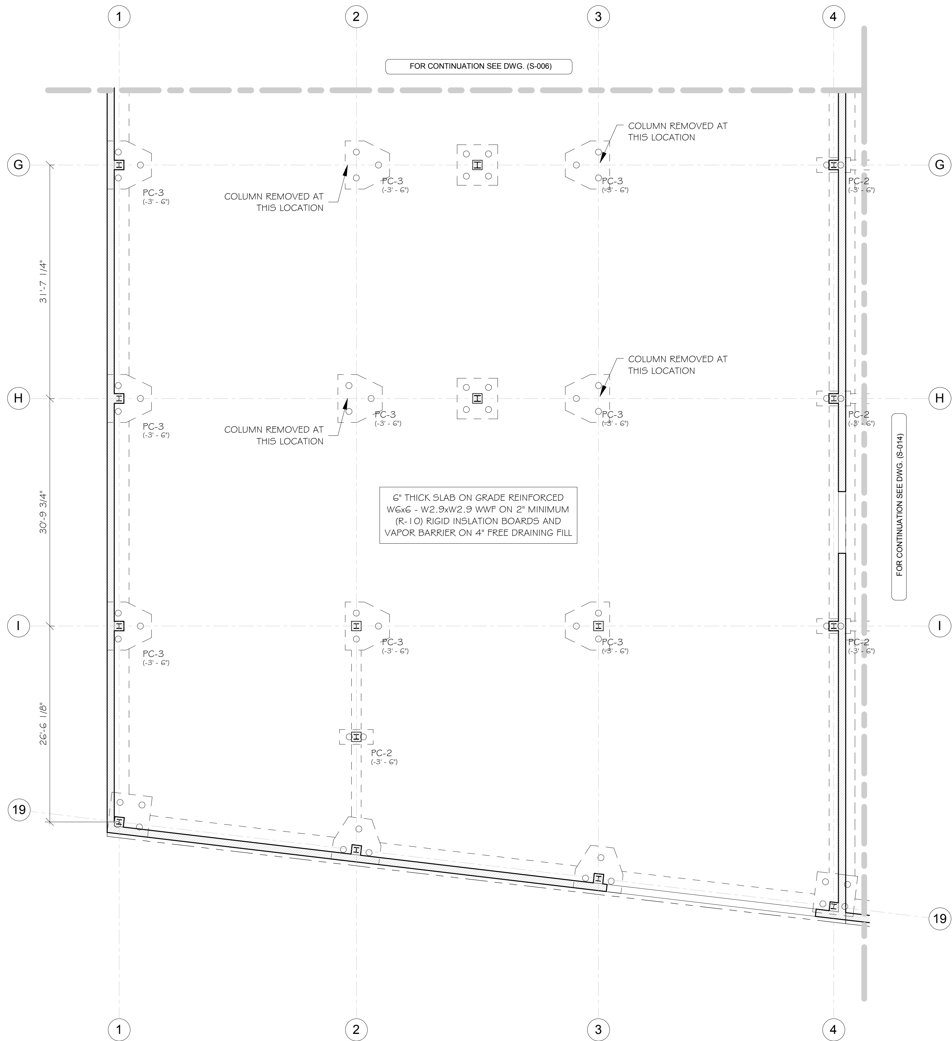
Partial - Proposed Slab on Grade and Pilecap Layout @ 537 Jonhson Ave (2 of 2):
